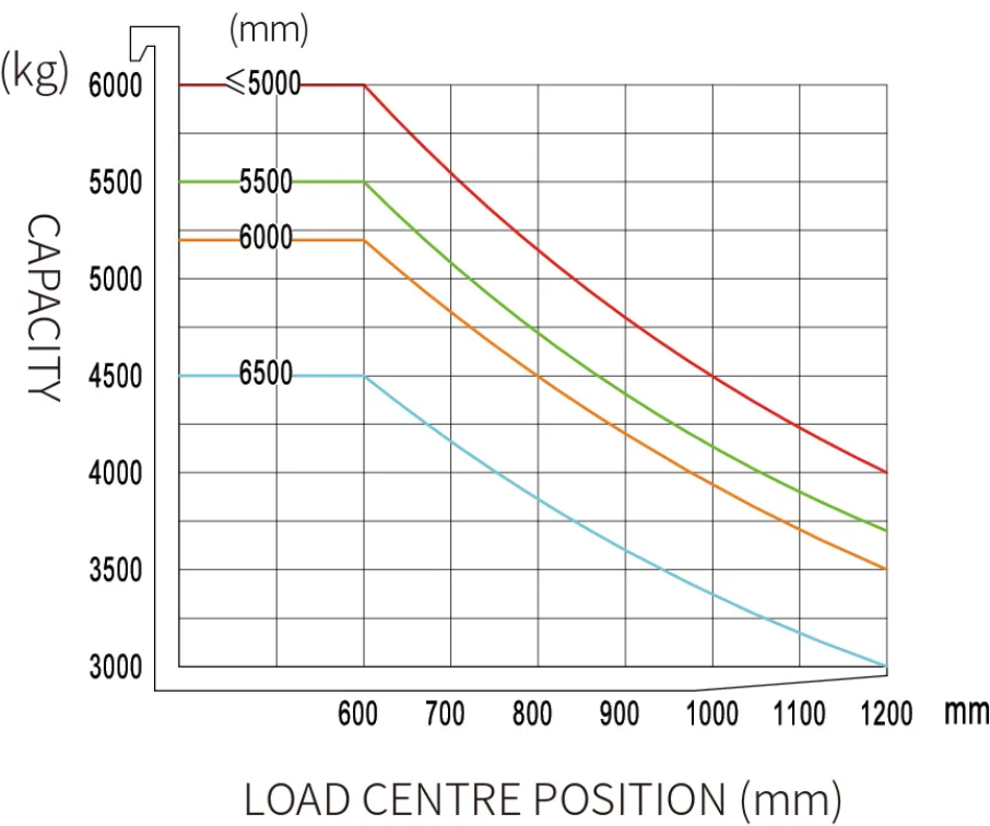
EFL603-HV-6 RATED CAPACITIES AND LOAD CENTERES GRAPH
